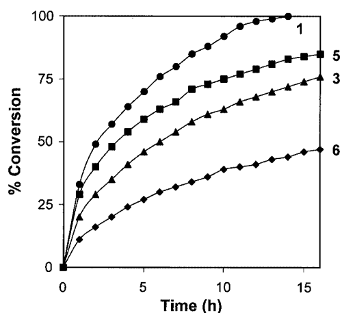
Figure 3. Comparative reaction rates for the metal-catalysed cyclisation of 4-pentyn-1-amine to 2-methyl-1-pyrroline using [\text{Rh}(\text{CO})_2(\text{mdd})]^+\text{BPh}_4^- ( 3 ) (▲), [\text{Rh}(\text{CO})_2(\text{mdd})]^+\text{PF}_6^- ( 5 ) (■), [\text{Rh}(\text{bim})(\text{CO})_2]^+\text{PF}_6^- ( 6 ) (◆), and [\text{Rh}(\text{bim})(\text{CO})_2]^+\text{BPh}_4^- ( 1 ) (●); catalyst loading 1.5% at 60 °C in [\text{D}_8]\text{THF} solution
