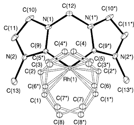
Figure 1. An ORTEP [10,11] depiction of the cation of [\text{Rh}(\text{cod})(\text{mdd})]^+\text{BPh}_4^- ( 2 ) showing 20% displacement ellipsoids and cod ligand disorder about a (pseudo) mirror plane (see main text and Exp. Sect.); atoms labelled with an asterisk are generated from the unique sites by x, 3/2 - y, z
