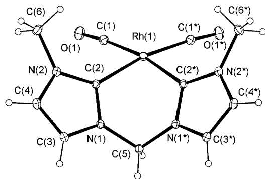
Figure 2. An ORTEP [10,11] depiction of the cation of [\text{Rh}(\text{CO})_2(\text{mdd})]^+\text{PF}_6^- ( 5 ) showing 20% displacement ellipsoids. Atoms labelled with an asterisk are generated from the unique sites by x, 1/2 - y, z .
